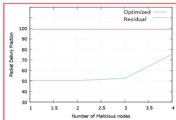
Figure 1 :- Packet Deliver Fraction of the Optimized buffere aware routing in comparison with the Residual Buffer aware routing
