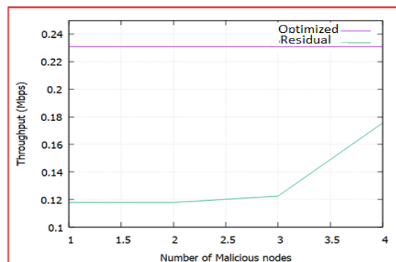
Figure 2 :- Throughput of the Optimized buffere aware routing in comparison with the Residual Buffer aware routing
