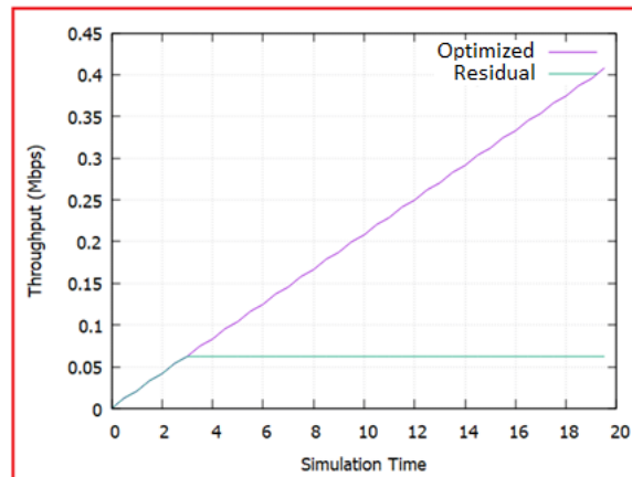
Figure 3 :- Throughput of the Optimized buffere aware routing in comparison with the Residual Buffer aware routing
