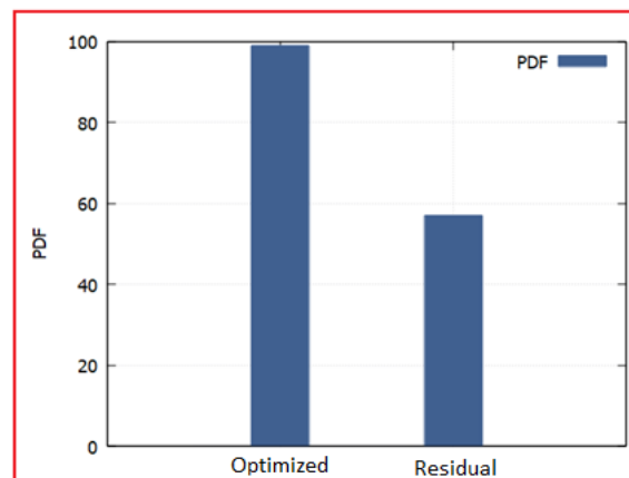
Figure 4 :- Overall packet delivery fraction comparison proposed work with the Residual Buffer aware routing
