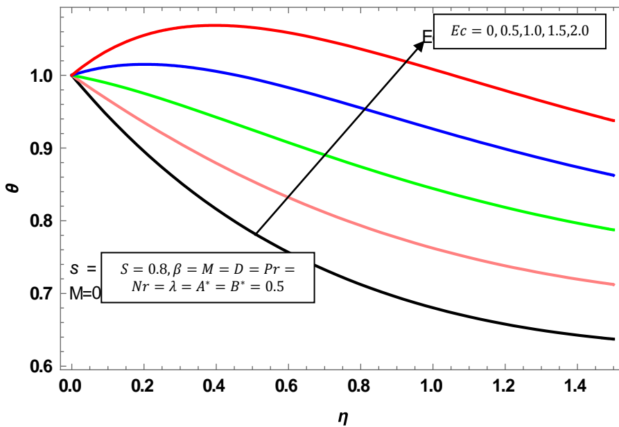
Fig.8. For S = 0.8 , impact of Ec , the Eckert number on \theta(\eta)
