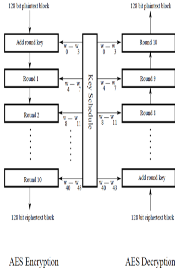
Fig. 7 AES Algorithm
