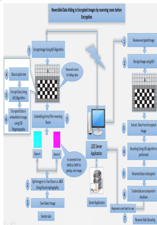
Fig.1 System Architecture
