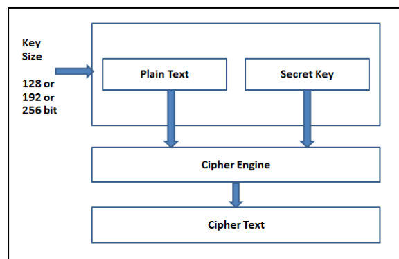
Fig 6.AES Blocks
