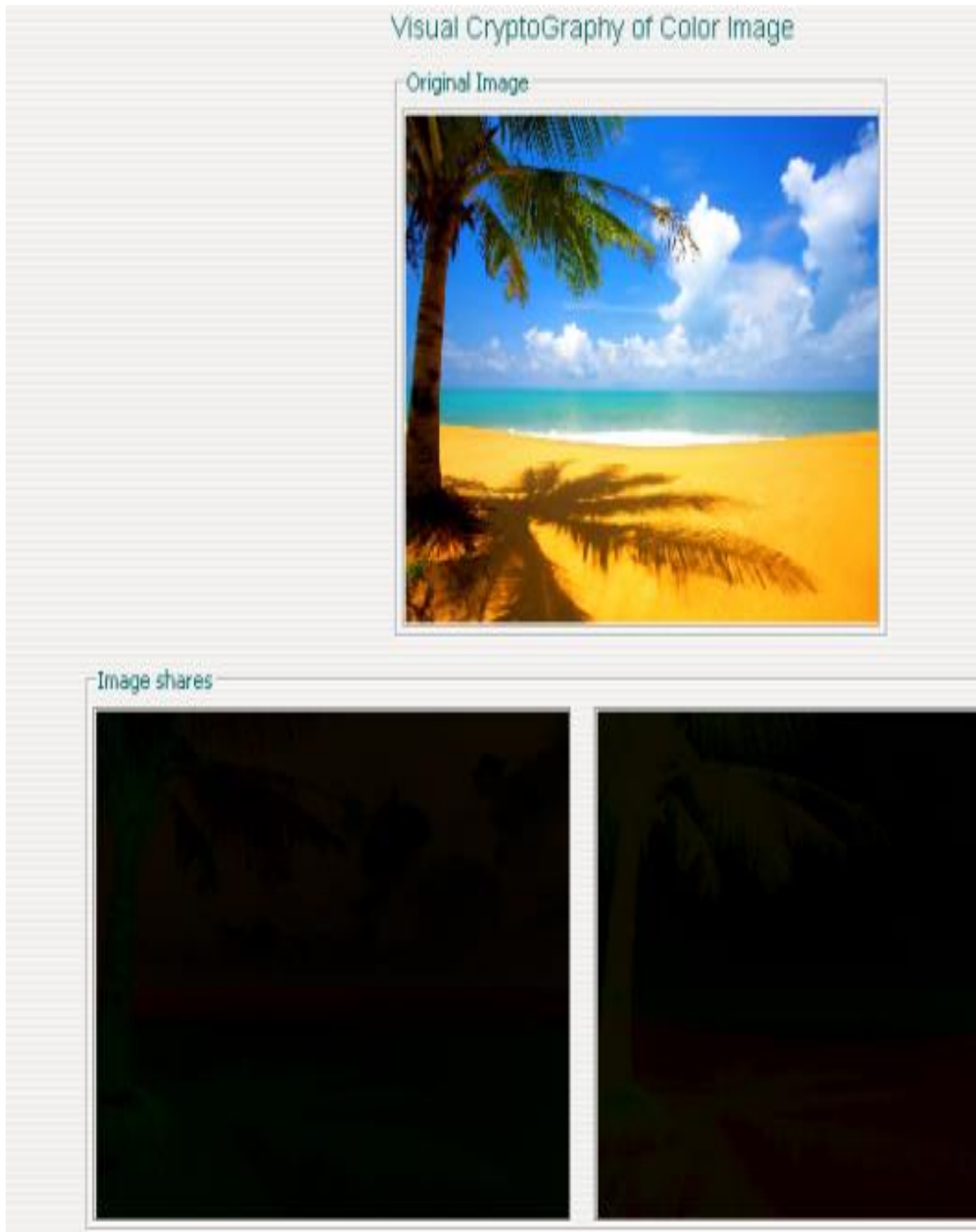
Fig.3 Image partition.
