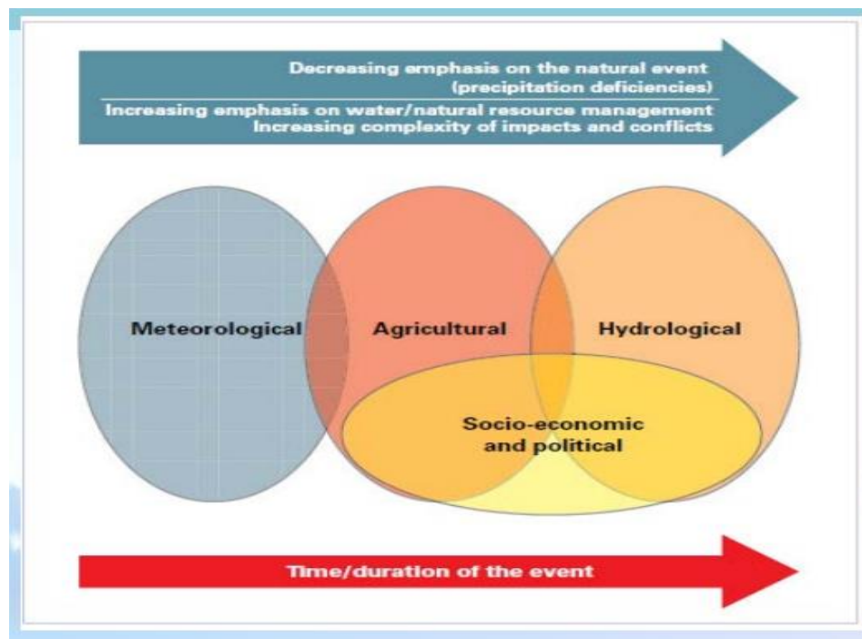
Fig 2: Interrelationships between meteorological, agricultural, hydrological and socio-economic drought.
