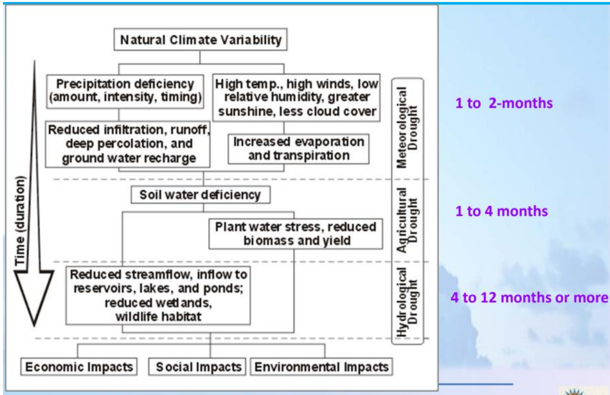
Fig 1: Type of drought and time response[1]
